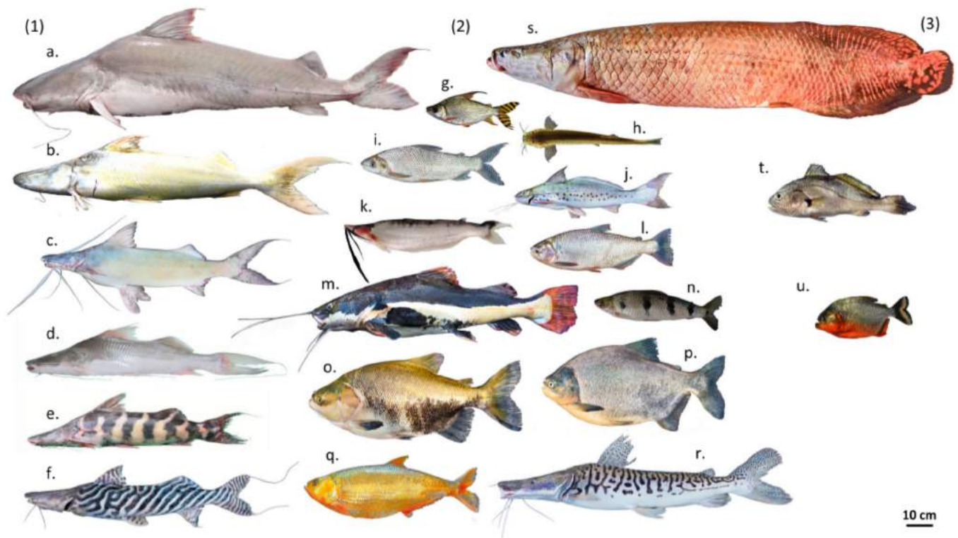
FIGURE 3 Examples of species belonging to the three main categories of migrations (most of which are cited in the text). (1) Long-distance migrations: (a) Brachyplatystoma filamentosum , (b) Brachyplatystoma rousseauxii , (c) Brachyplatystoma platynemum , (d) Brachyplatystoma vaillantii , (e) Brachyplatystoma juruense , (f) Brachyplatystoma tigrinum . (2) Medium-distance migrations: (g) Semaprochilodus insignis , (h) Trichomycterus barbouri , (i) Prochilodus nigricans , (j) Calophysus macropterus , (k) Hypophthalmus fimbriatus , (l) Brycon amazonicus , (m) Phractocephalus hemiliopterus , (n) Schizodon fasciatus , (o) Colossoma macropomum , (p) Piaractus brachipomus , (q) Pellona flavipinis , (r) Pseudoplatystoma tigrinum . (3) Short-distance migrations: (s) Arapaima sp., (t) Plagioscion squamosissimus , (u) Pygocentrus nattereri . For the sake of available space and visibility of small species, large species reaching over 1 m lengths (a, b, l, q, r, s) are not represented to their maximum length, unlike small and medium species. The scale does not apply to T. barbouri (h), given its very small size at migration (~30 mm). Photo credits: (a), (d), (e) García Dávila et al. (2018); (b) Fernando Carvajal-Vallejos; (c), (f), (i), (j), (l), (m), (o), (p), (r) Aldo Echeverría; (h) Guido Miranda (WCS); (g), (k), (n), (t)–(w) Arantes, Winemiller, et al. (2019); (q), (s) Daniel Barroso
